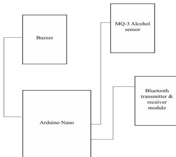
Fig (1) Block diagram of motorcycle security system
