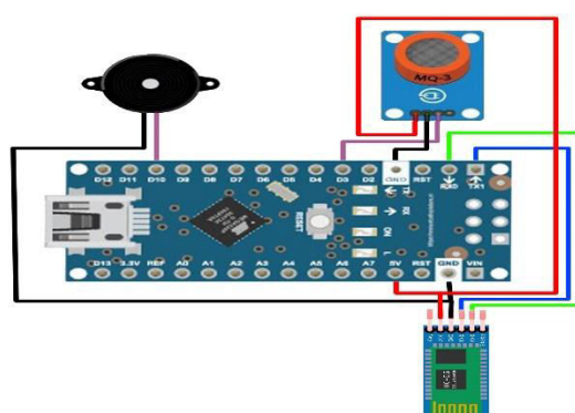
Fig (4) Circuit diagram of smart helmet
