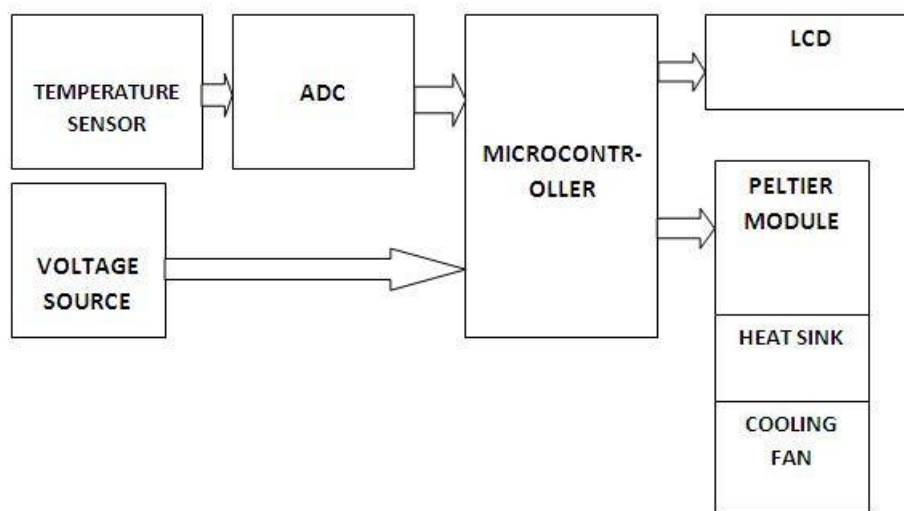
Fig 2. Block Diagram of system
