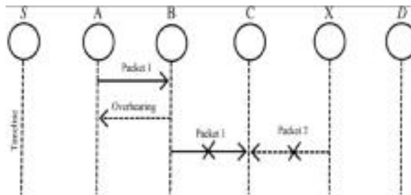
Fig. 3.1. Receiver Collisions occurs at receiver C because both nodes B and X are trying to send packets at same time. In above figure: S=Source, D=Destination and A, B, C...X=Nodes which shown the example of receiver collision in which after Node A packet 1 sends to the Node B, it tries to spy if Node B forwarded this packet to Node C, for the moment Node X is forwarding packet 2 to Node C. In such case, Node A spy that Node B has successfully delivered packet 1 to Node C but unable to detect that node C did not accept the packet due to a collision between packet 1 and packet 2 at Node C.
