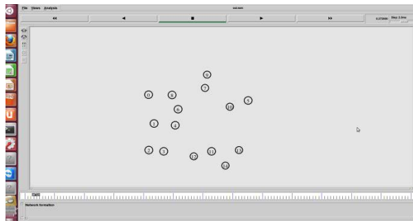
Fig 5. 1. Network formation
