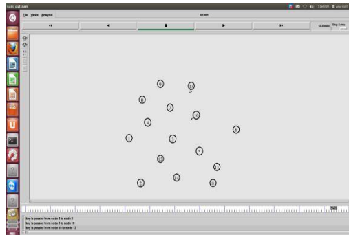
Fig 5.2.Key generation
