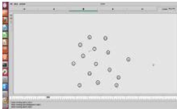
Fig 5.3. Acknowledgement Implementation
