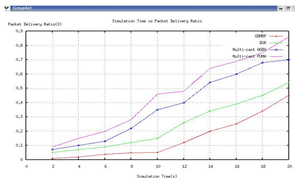
Fig:4 packet delivery ratio
