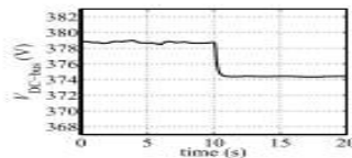
Case B: dc bus voltage profile.
