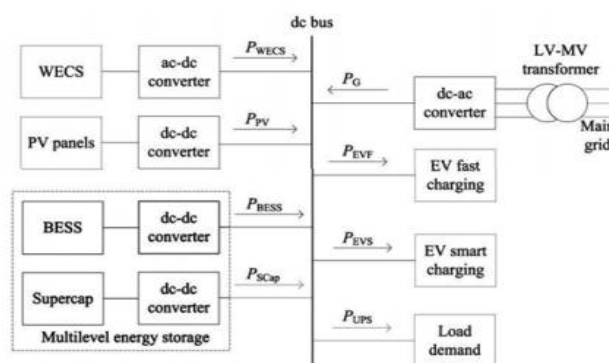
Fig:1 Outline diagram of the dc micro grid
