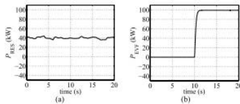
Case study: Assumptions of the simulation. (a) Renewable power generation. (b) Fast charging load connected to the dc bus.
