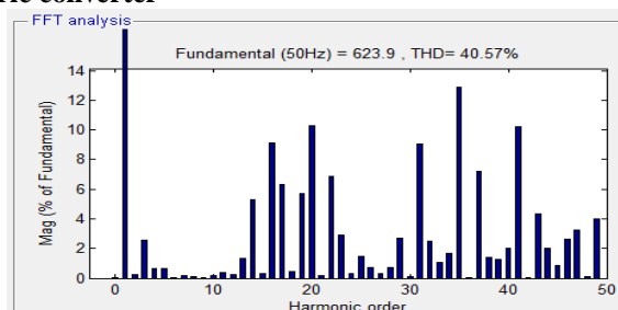
Fig-9 THD of the 4-level converter
