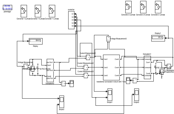
Fig-12 MATLAB/Simulink Model of nine-level dual converter based STATCOM
