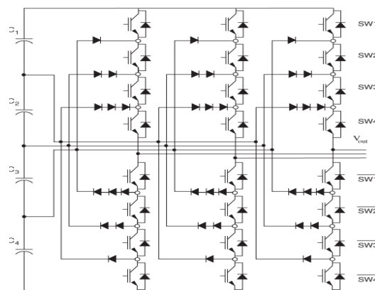
Fig-10 Three phase 9-level DCMLI circuit
