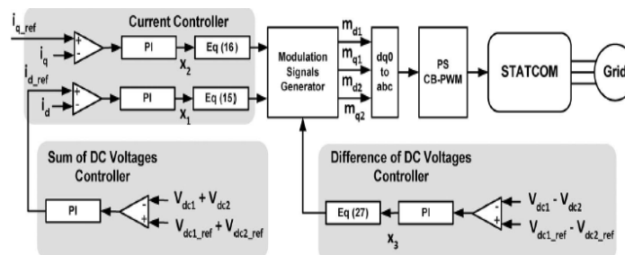
Fig-4 Controller Circuit of Statcom
