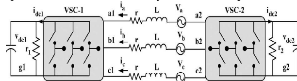
Fig-3 Equivalent circuit diagram of the proposed STATCOM
