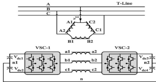
Fig-1 Transformer based four level statcom
