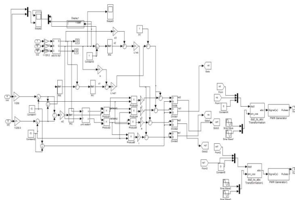
Fig-6 MATLAB/Simulink Model diagram of the controller
