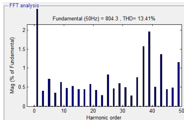
Fig-14 Shows the THD of the DCMLI
