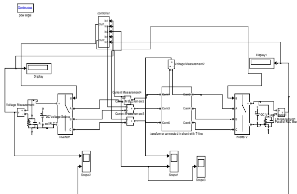
Fig-5 MATLAB/Simulink Model Circuit of asymmetric Dual converter base Statcom
