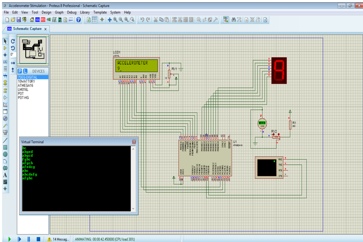
Fig.4. Simulation Result in Proteus software
