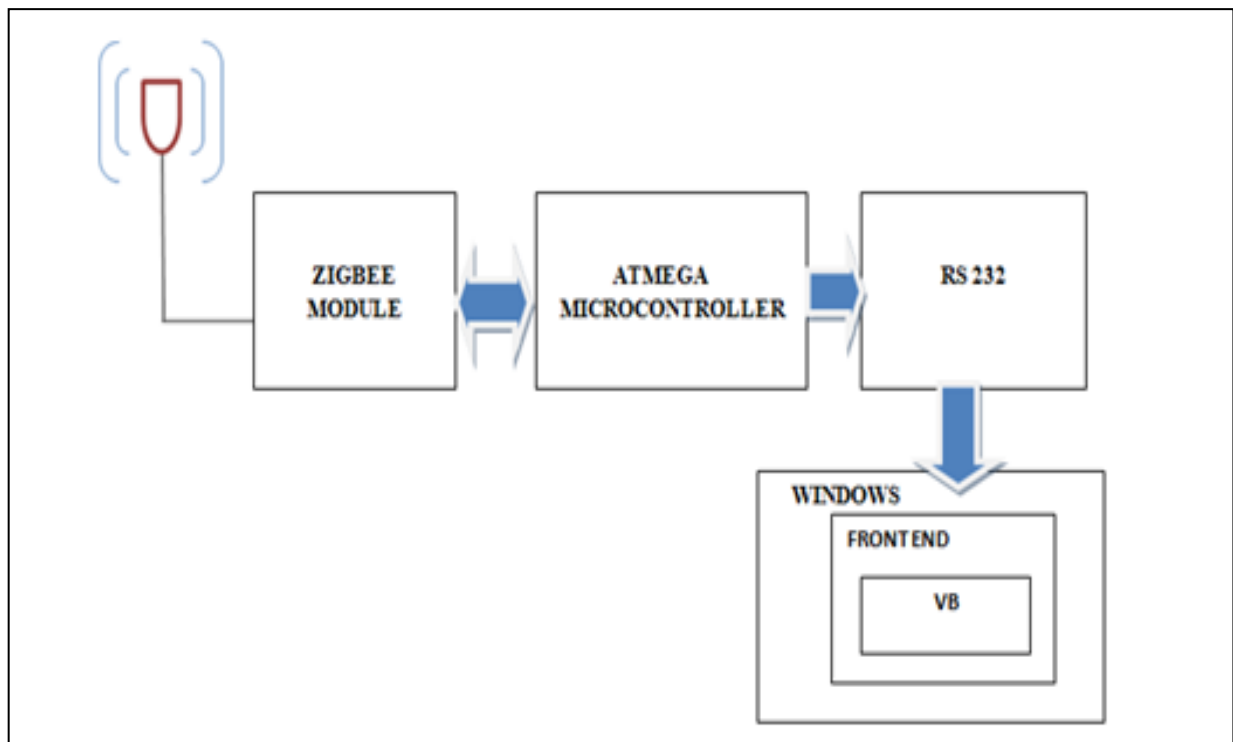
Fig.2. Block Diagram for Receiver Section
