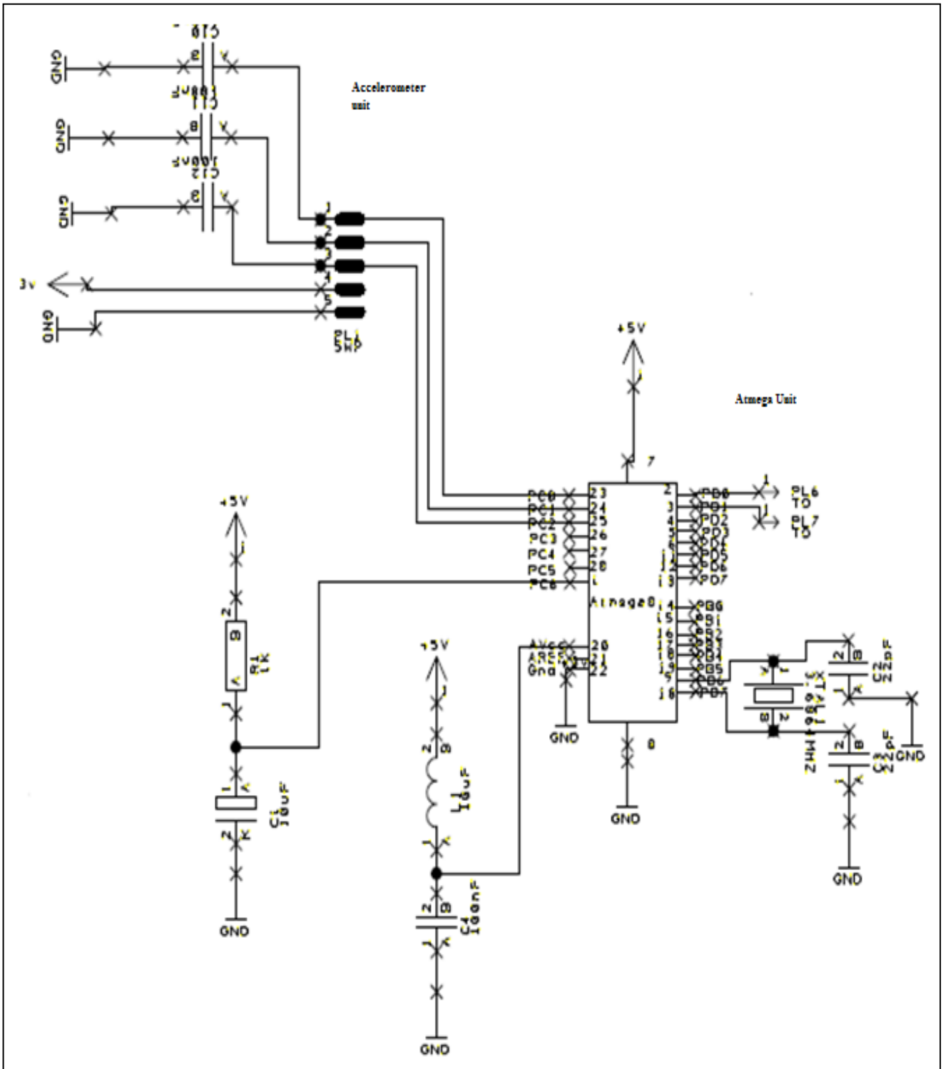
Fig.3. Schematic Diagram for MEMS based device
