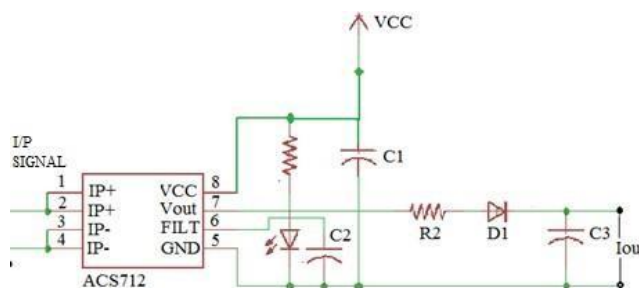
Fig.3: Current Sensor Diagram
