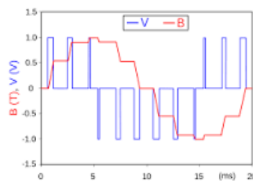
Figure 5: PWM Diagram
