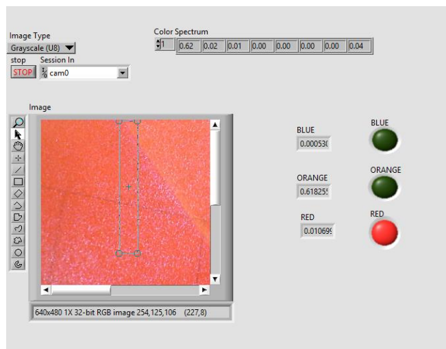
Figure 9: Front Panel for Red color
