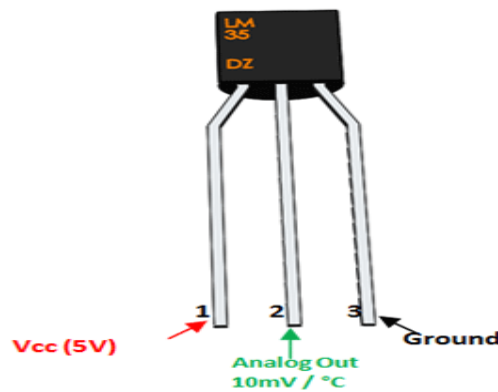
Fig 3:- Temperature sensor
