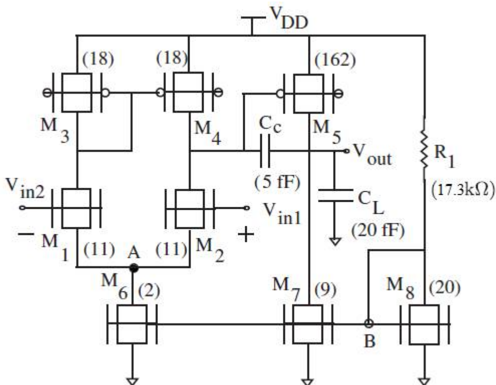
Fig. 2: Finfet based compensation Op-Amp.
