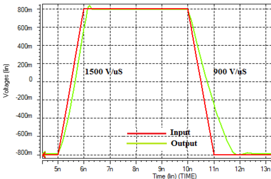
Fig. 5: Zoomed simulation waveform for Slew Rate measurement
