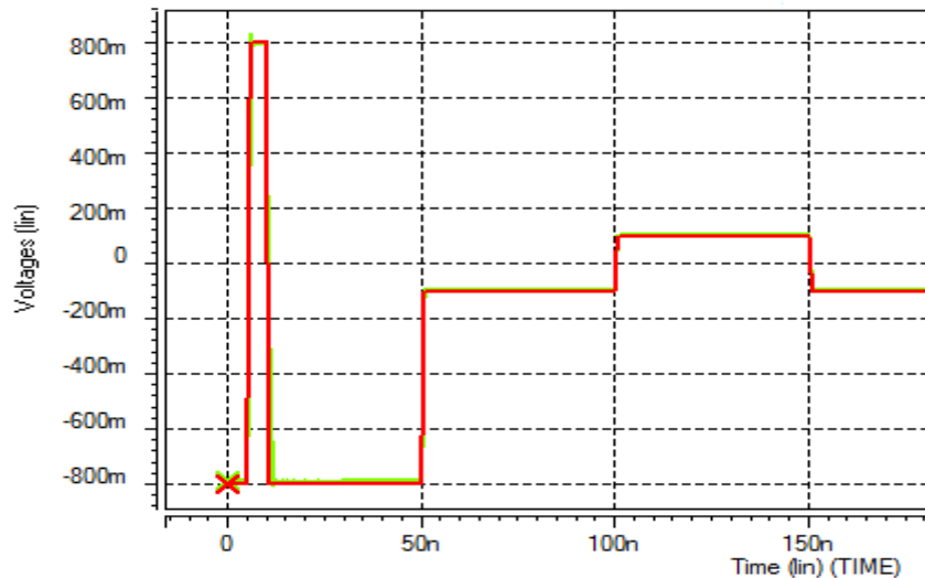
Fig. 4: Simulation waveform for transient analysis for slew rate measurement
