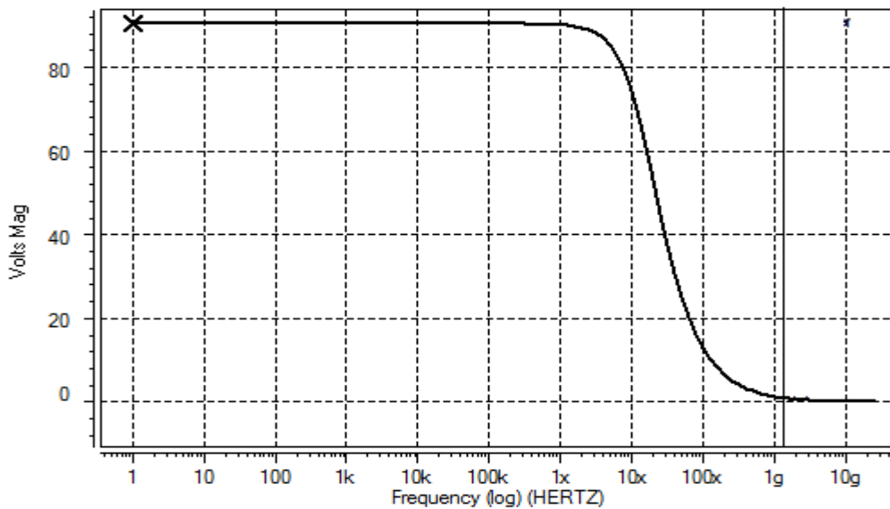
Fig. 6: Gain Vs Frequency Plot of proposed Op-Amp
