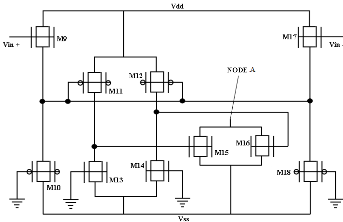
Fig. 3: Dynamic Bias Circuit
