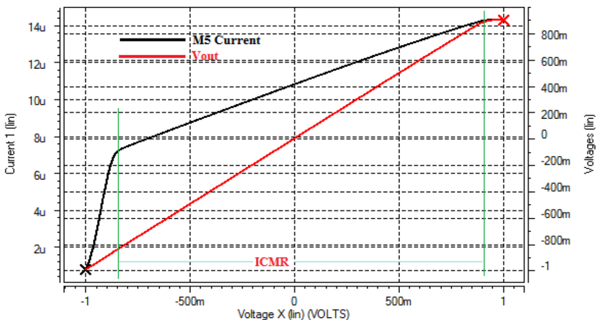
Fig. 7: ICMR calculation of proposed Op-Amp
