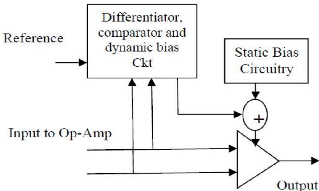
Fig. 1: Block Diagram of proposed High Slew Rate Op-amp
