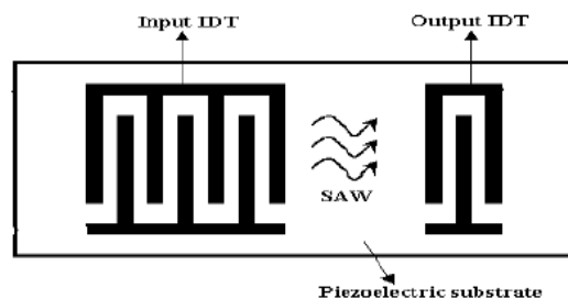
Fig. 1. SAW Device
