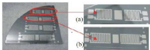
Fig. 12. Conventional SAW Biosensor a) IDT with 10 fingers, b) IDT with 16 fingers.
