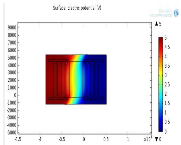
Fig. 7. Potential Flow
