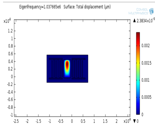
Fig. 10. Displacement Flow
