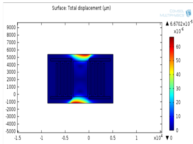
Fig. 6. Displacement Flow
