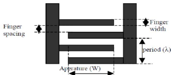
Fig. 2. IDT Structure
