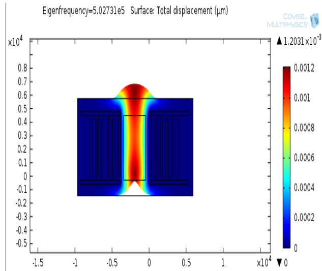
Fig. 8. Displacement Flow
