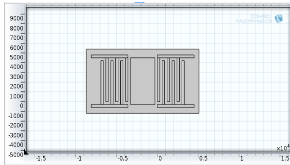
Fig. 5. Design of SAW Device
