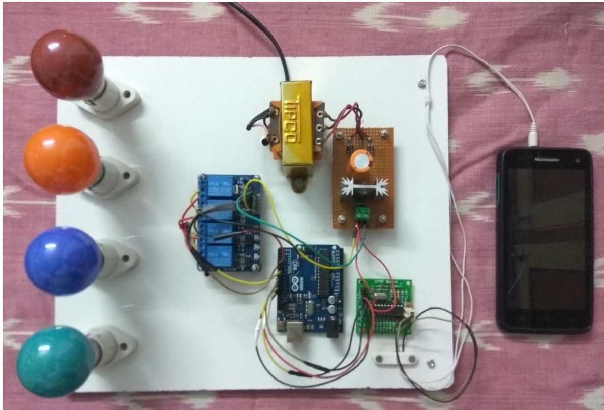
Fig. 7: Assembled Model
