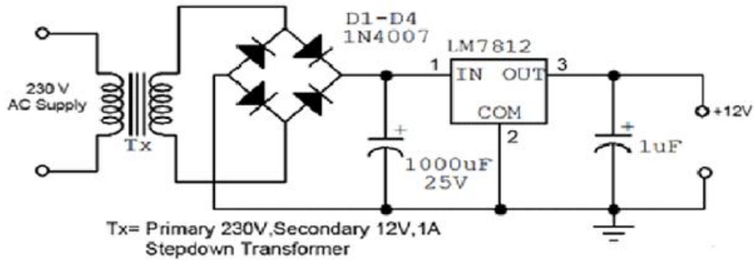
Fig. 1: Power Supply circuit
