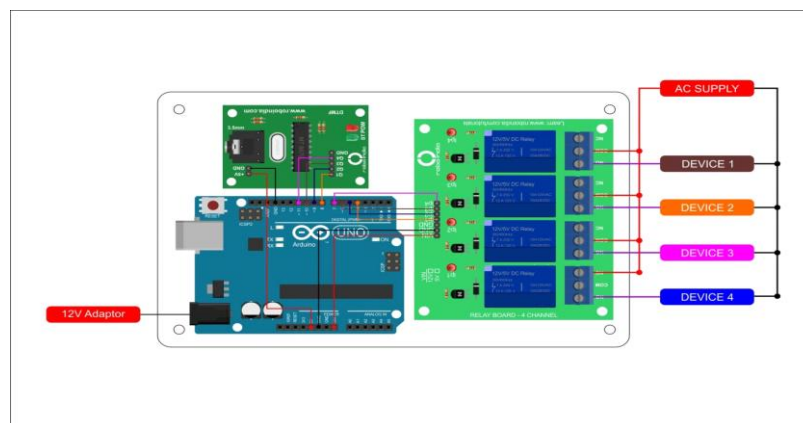
Fig. 6: Connection layout of the hardware
