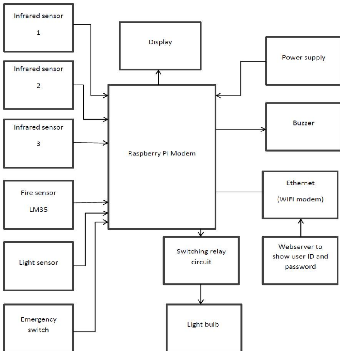
Fig 1. Block diagram of system
