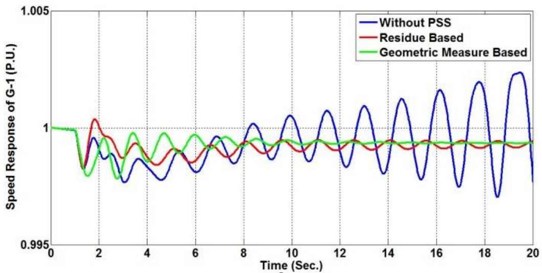
Fig. 7 Speed response of generator – 1
