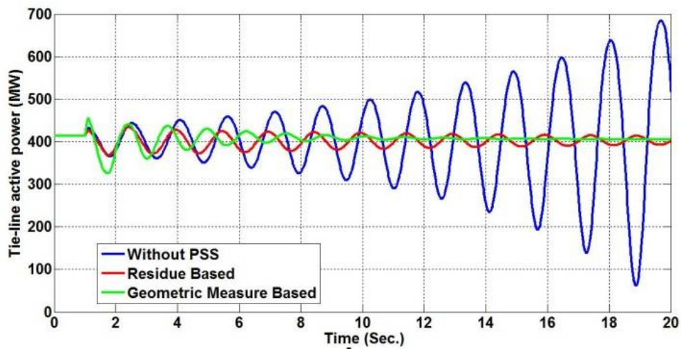
Fig. 6 Tie line active power flow deviation
