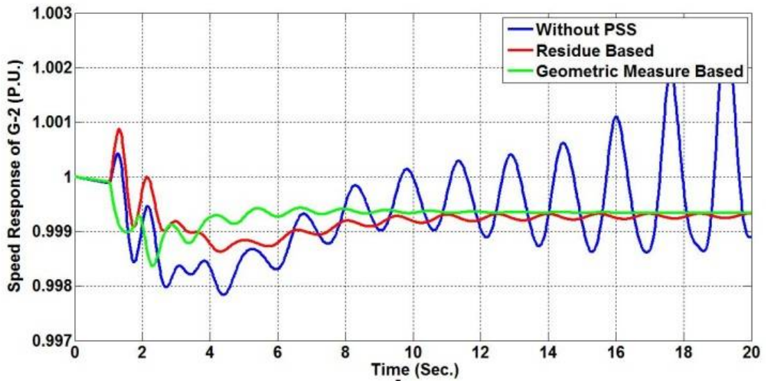
Fig. 8 Speed response of generator – 2
