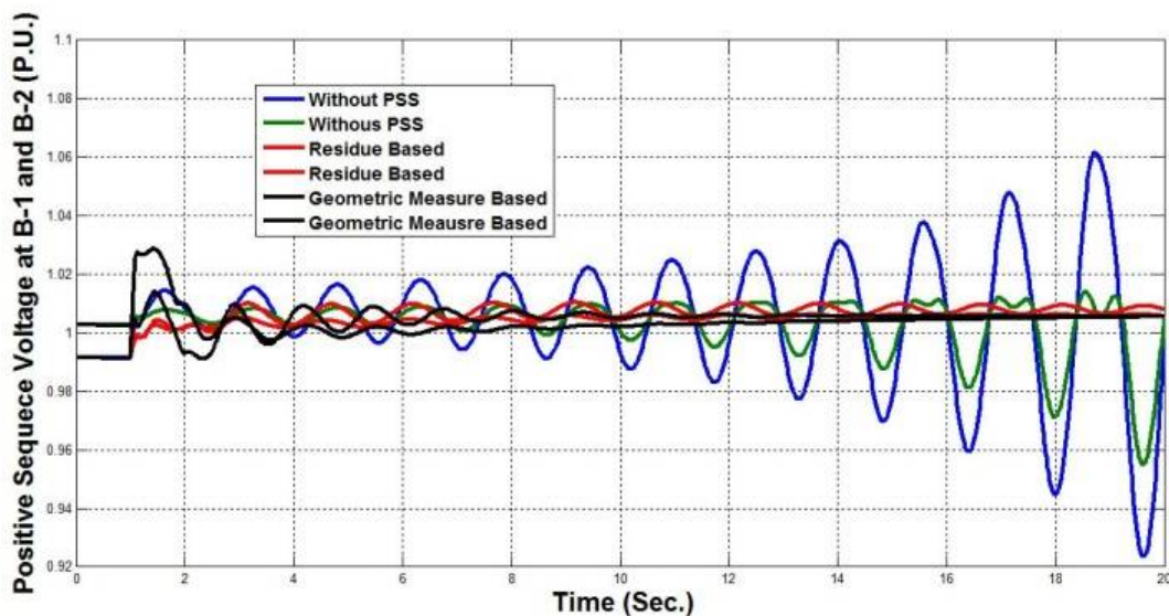
Fig. 10 Positive sequence voltage at Bus-1 and Bus-2
