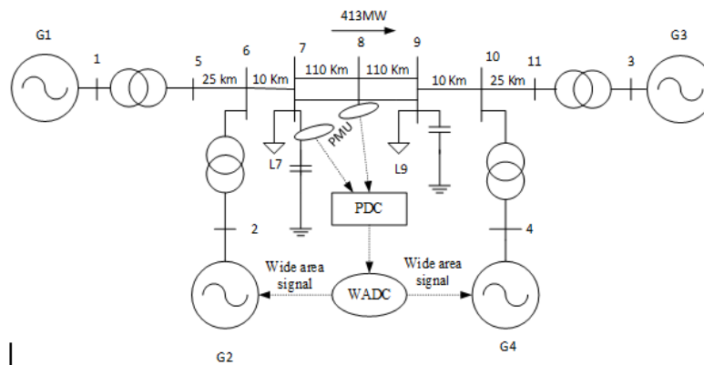
Fig-5Kundur's Two Area Four Machine System
