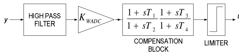
Fig-3 Conventional Power System Stabilizer
