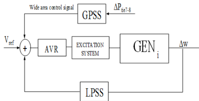
Fig. 4Global area control scheme.
