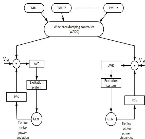
Fig. 1 General structure of wide area damping controller
