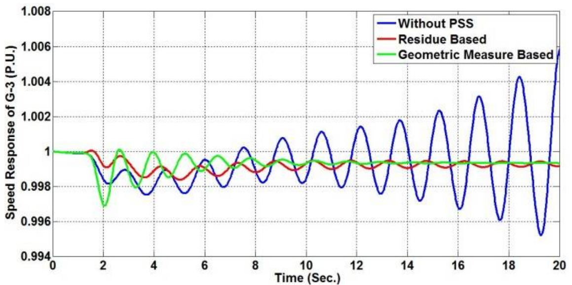
Fig. 9 Speed response of generator – 3
