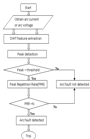
Fig. 5 Flowchart for series arc fault detection using DWT
