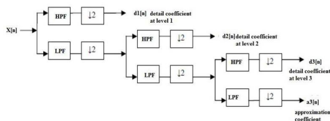
Fig.4 Three level decomposition of a signal
