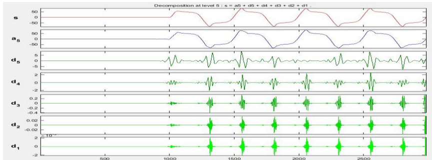
Fig.8(a) Five level decomposition using symlet
