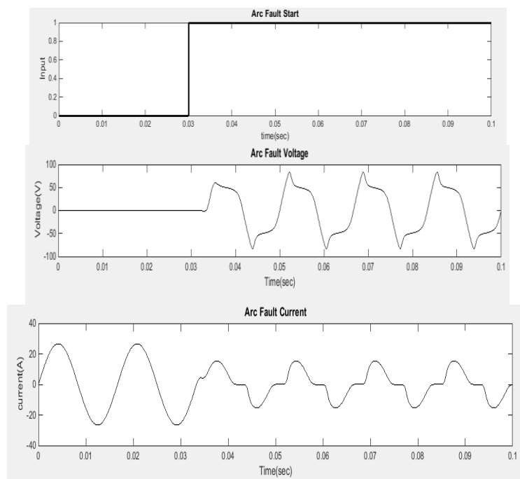
Fig. 6 Series arc-fault simulation results.
