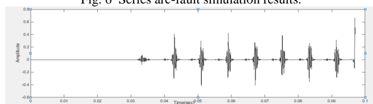
Fig. 7 Series arc-fault feature extraction using DWT and db4.
