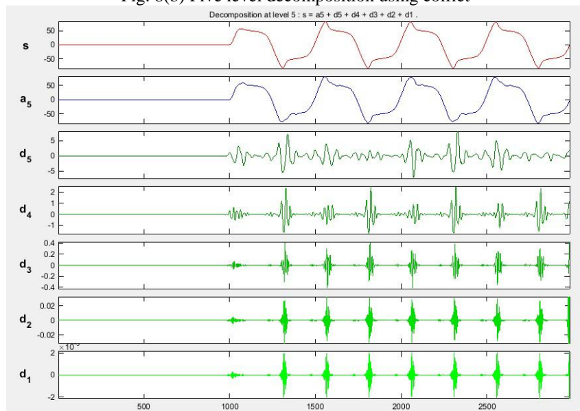
Fig.8(c) Five level decomposition using daubechies
