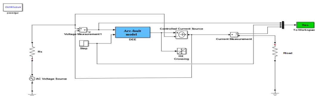
Fig. 3 Series arc-fault simulation model
