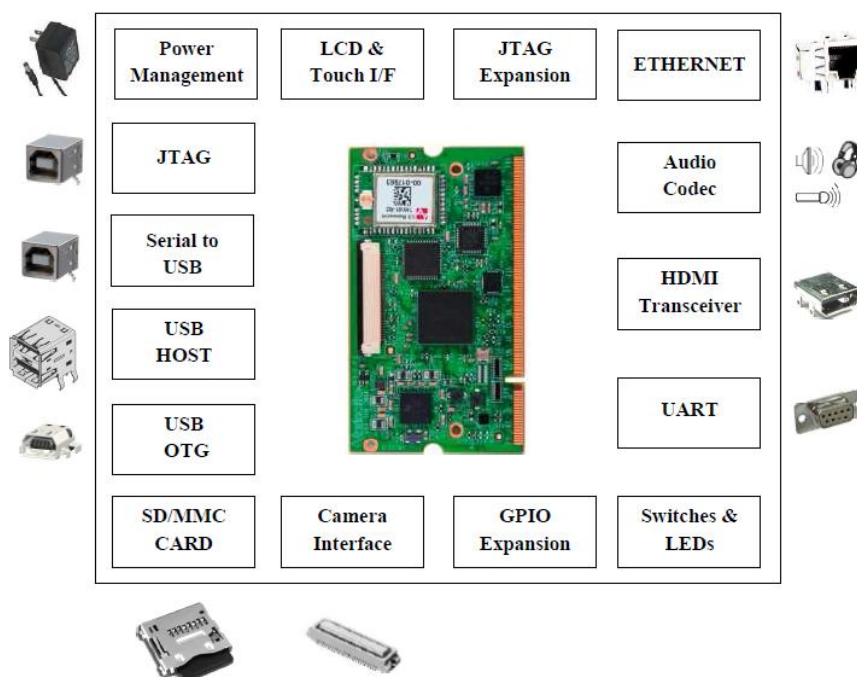
Fig 1: block diagram of OMAP4460 development board.
