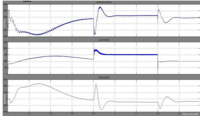
Figure 4: Power balancing conditions
