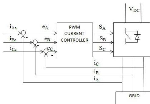
Figure 2: Current control pulse width modulation technique.
