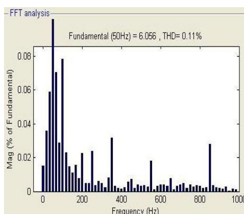
Figure 7: Total harmonic distortion values
