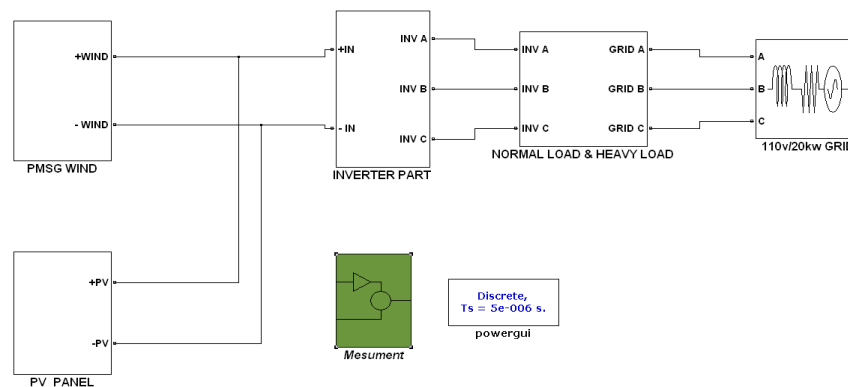
Figure 3: Main model of grid connected system
