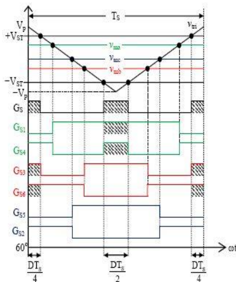
Fig.4. Gate control signal for SBI for \omega t=60^\circ
