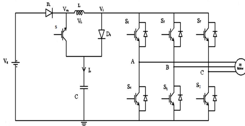
Fig.1. Schematic of three phase SBI
