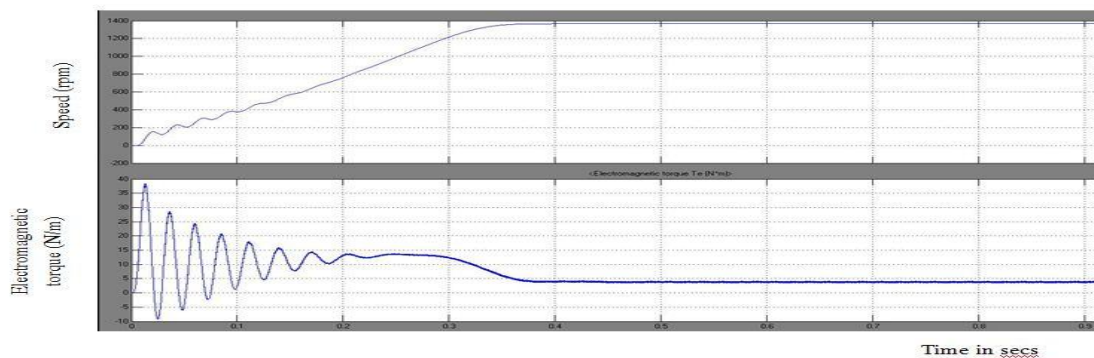
Fig.7. Waveform of speed and torque of a induction motor controlled by V/F method
