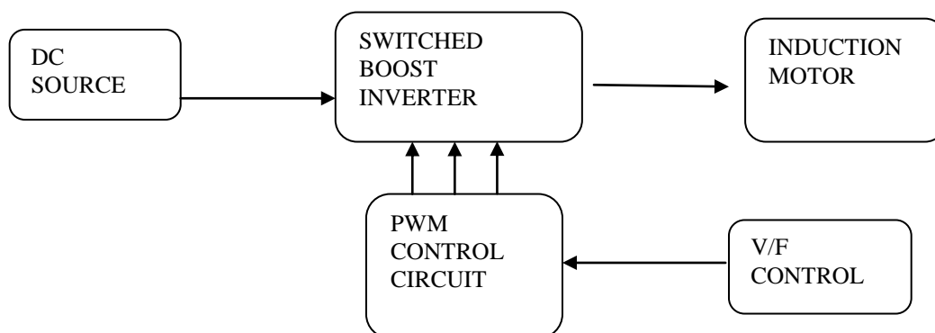
Fig.1: Block diagram of open V/F control of an induction motor fed by SBI
