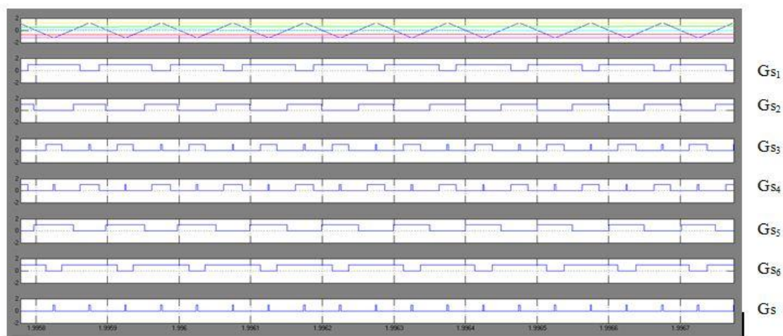
Fig.6. PWM control signals for \omega t=60^\circ
