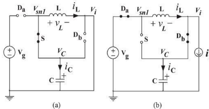
Fig.2. (a) Equivalent circuit diagram of SBI during the interval DT_s (b) Equivalent circuit diagram of SBI during the interval (1-D)T_s
