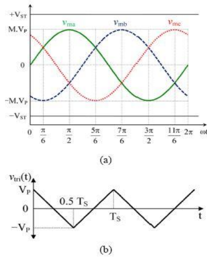
Fig.3. (a) The five modulation signals ( v_{ma} , v_{mb} , v_{mc} , +V_{ST} , -V_{ST} ) (b) The triangular carrier signal ( v_{tri} ) used for the gate control signal generation of the three-phase SBI
